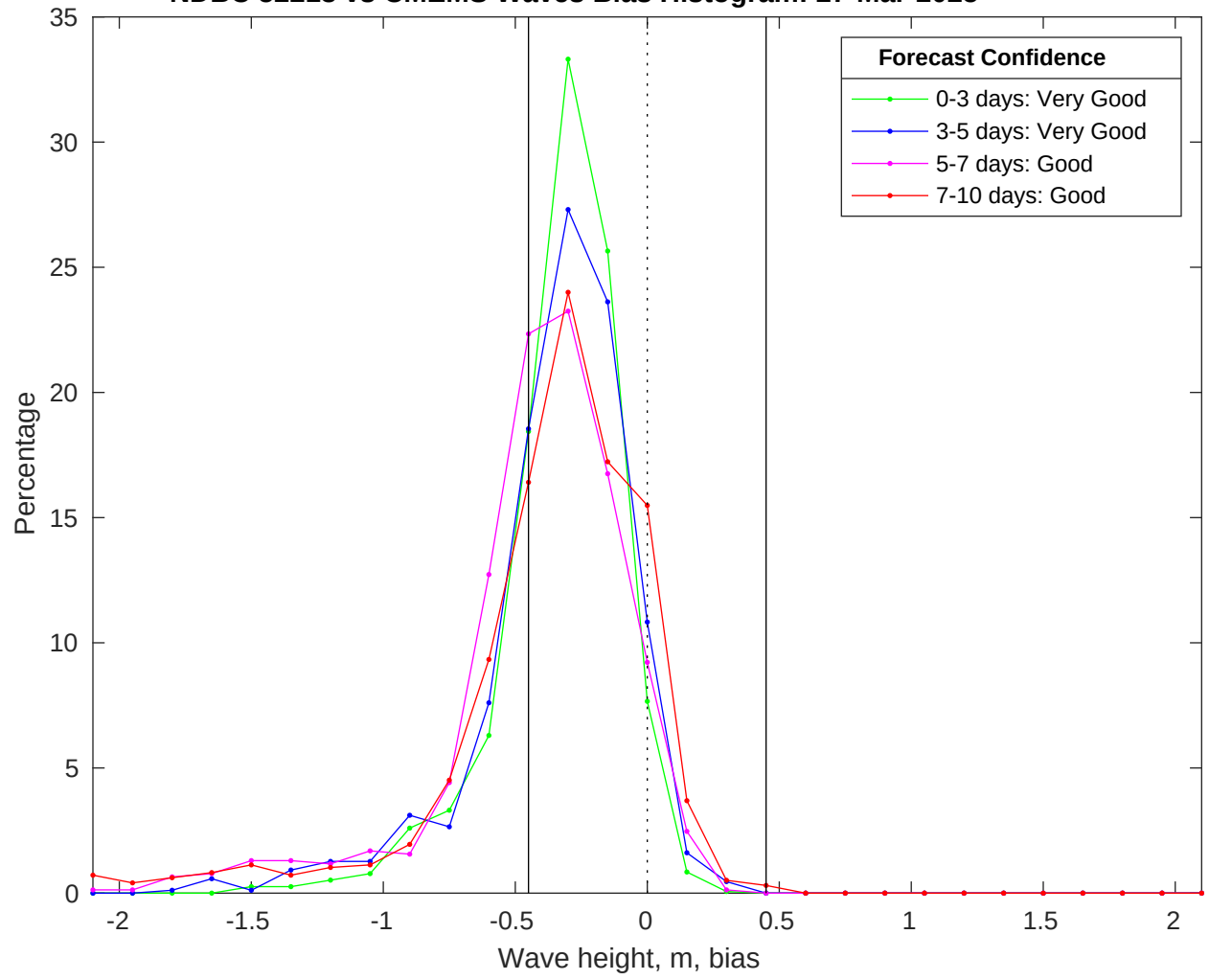
NDBC 52213 vs CMEMS Waves Bias Histogram: 27-Mar-2025
