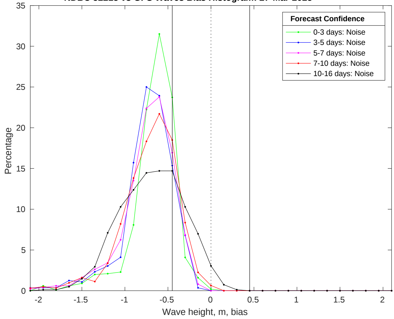
NDBC 52213 vs GFS Waves Bias Histogram: 27-Mar-2025
