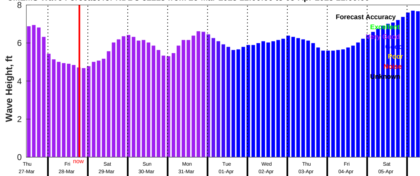
CMEMS Wave Forecast for NDBC 52213 from 26-Mar-2025 11:00:00 to 05-Apr-2025 11:00:00
