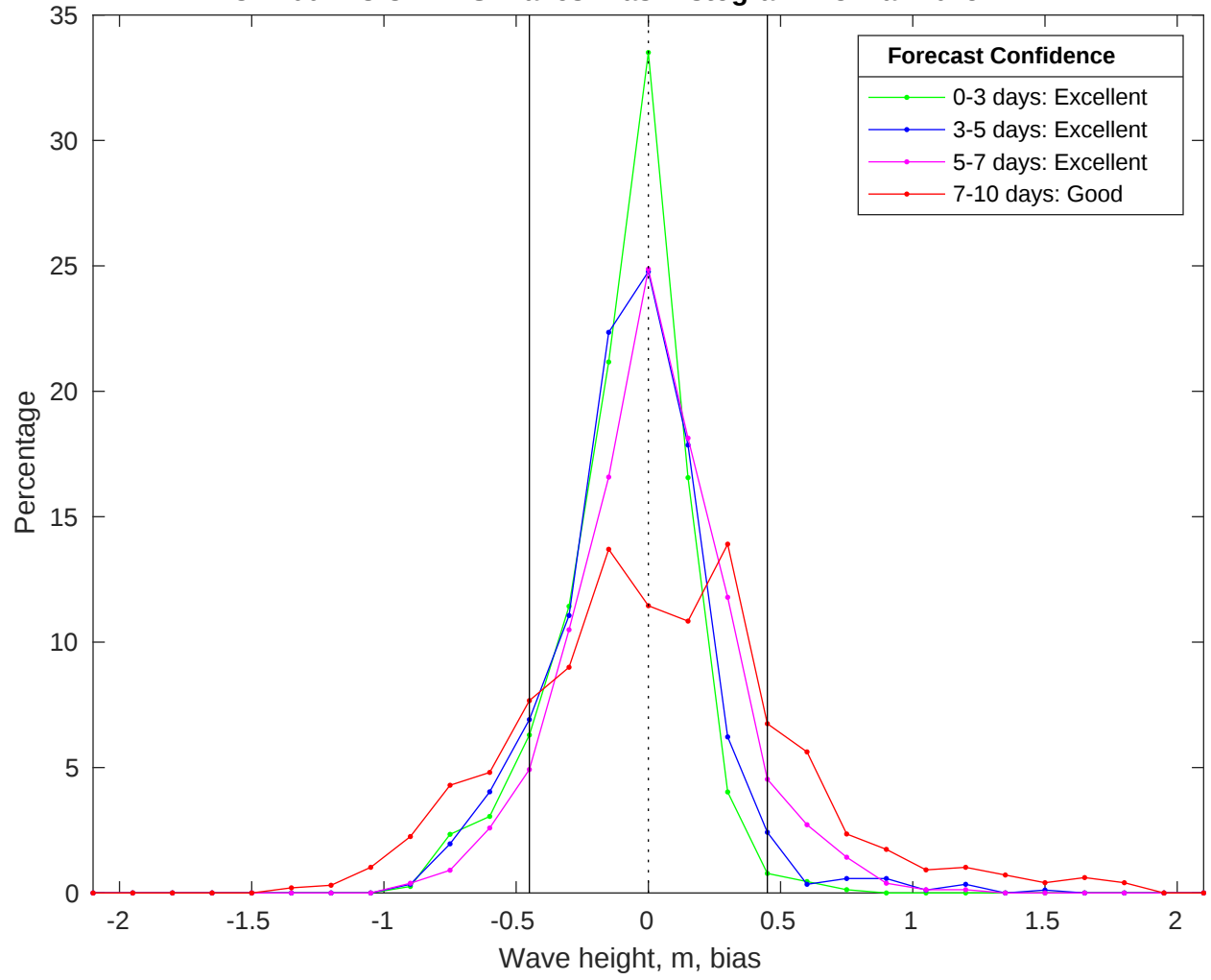
NDBC 41004 vs CMEMS Waves Bias Histogram: 28-Mar-2025
