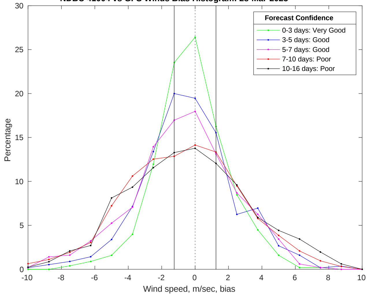
NDBC 41004 vs GFS Winds Bias Histogram: 28-Mar-2025
