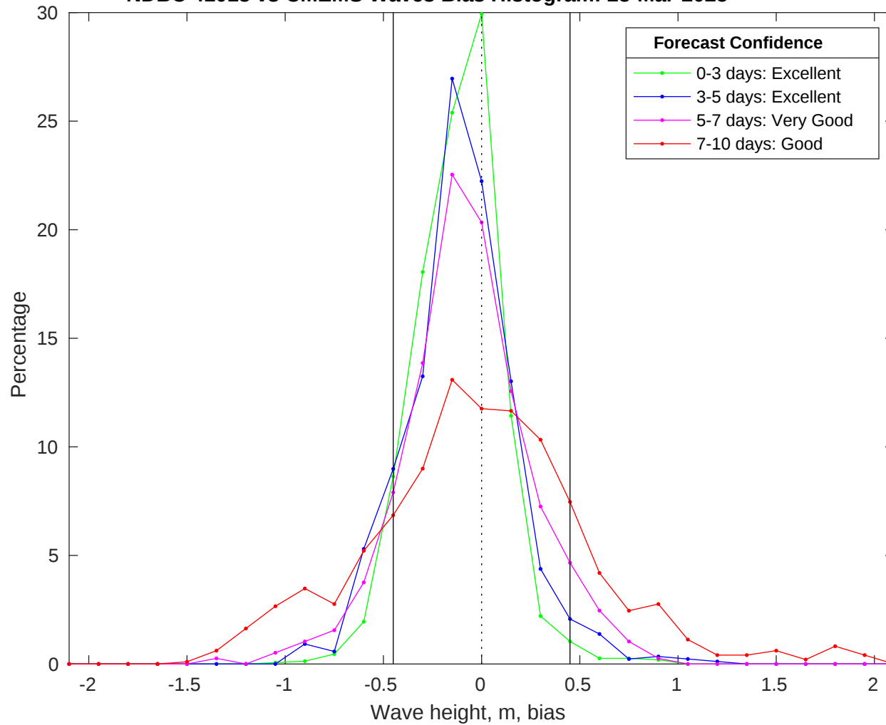
NDBC 41013 vs CMEMS Waves Bias Histogram: 28-Mar-2025
