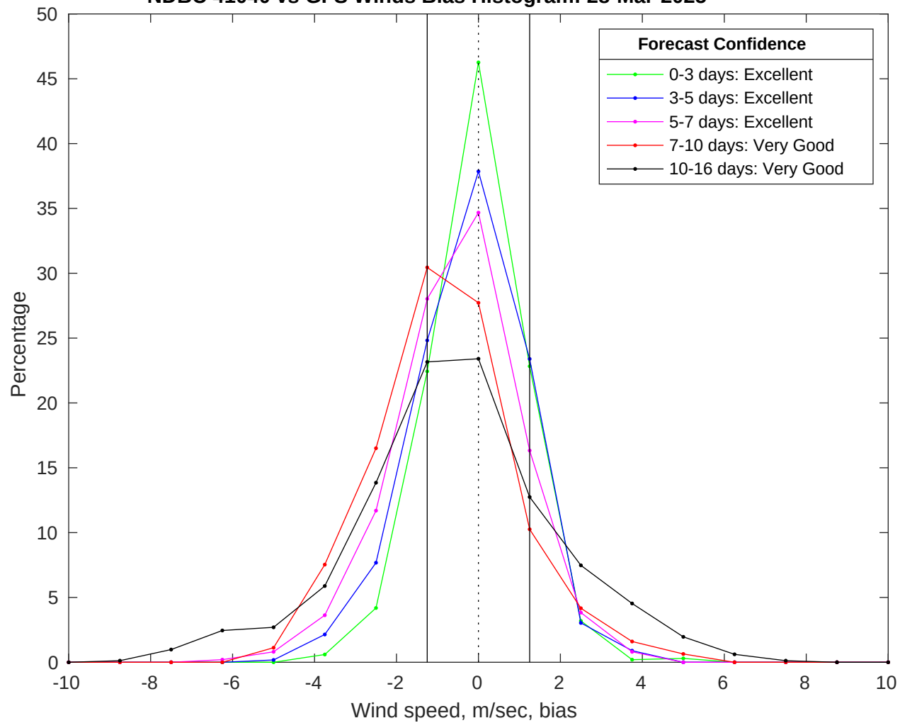
NDBC 41040 vs GFS Winds Bias Histogram: 28-Mar-2025
