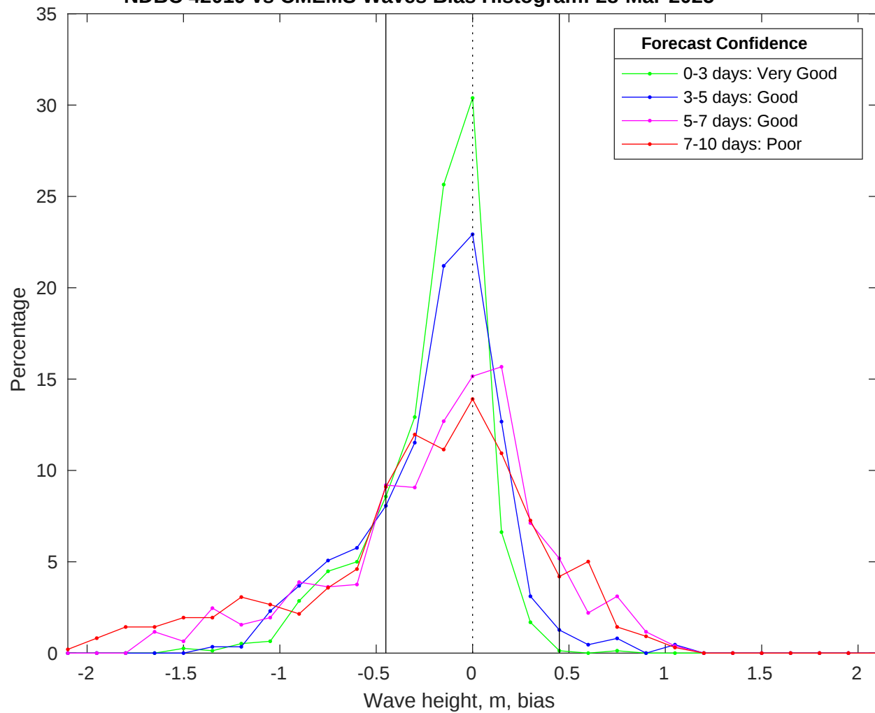
NDBC 42019 vs CMEMS Waves Bias Histogram: 28-Mar-2025
