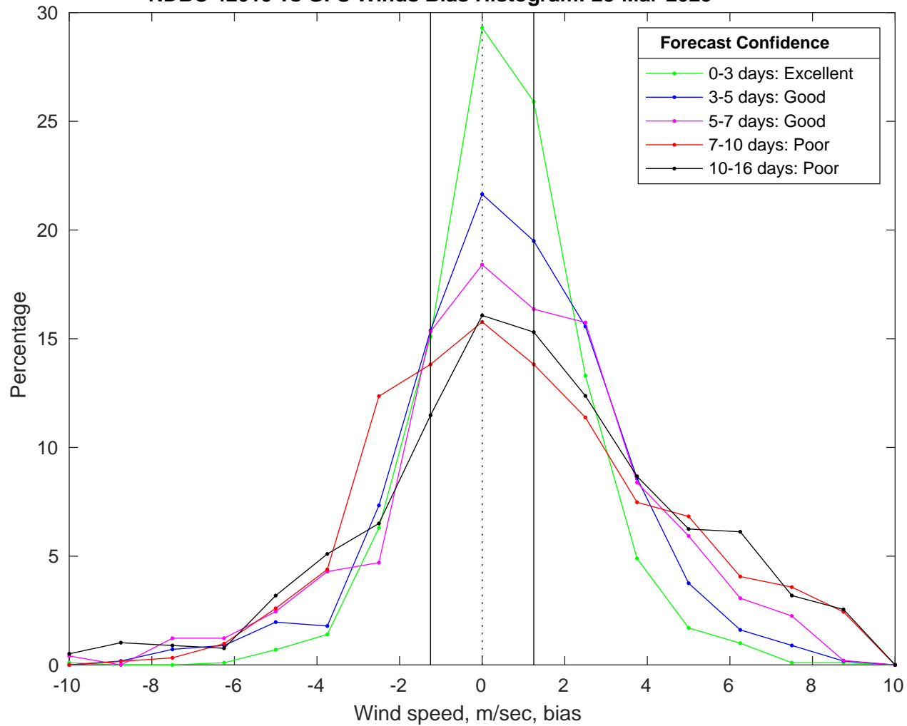
NDBC 42019 vs GFS Winds Bias Histogram: 28-Mar-2025
