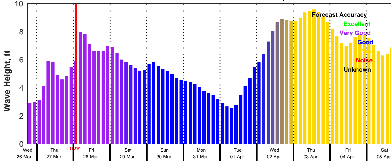
CMEMS Wave Forecast for NDBC 42019 from 26-Mar-2025 18:00:00 to 05-Apr-2025 18:00:00
