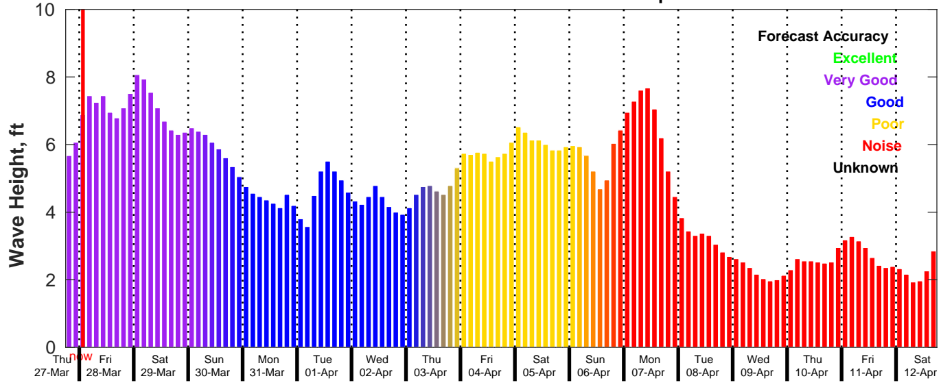
GFS Wave Forecast for NDBC 42019 from 27-Mar-2025 18:00:00 to 12-Apr-2025 18:00:00
