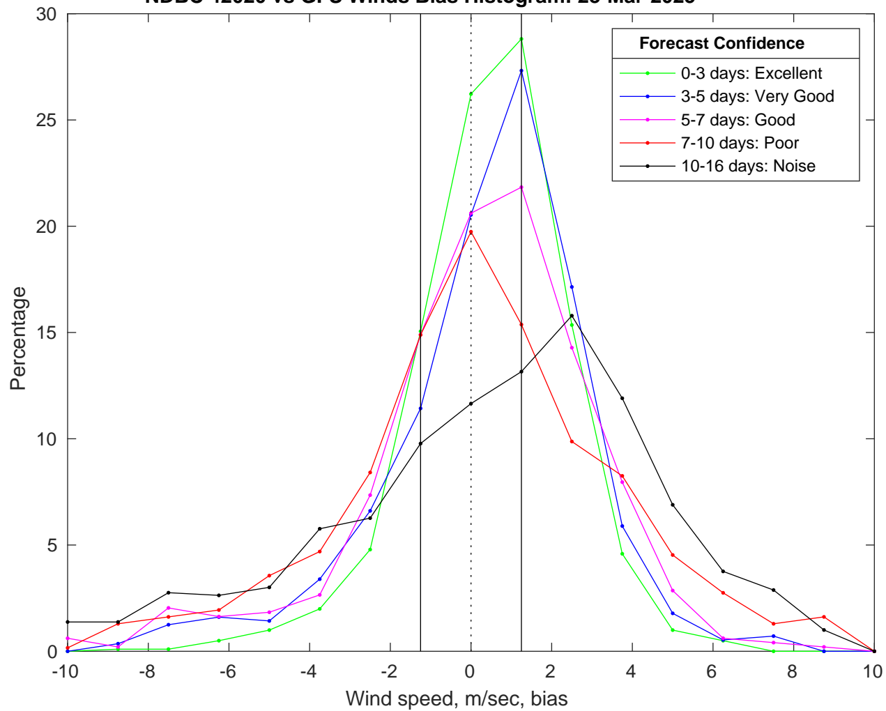
NDBC 42020 vs GFS Winds Bias Histogram: 28-Mar-2025
