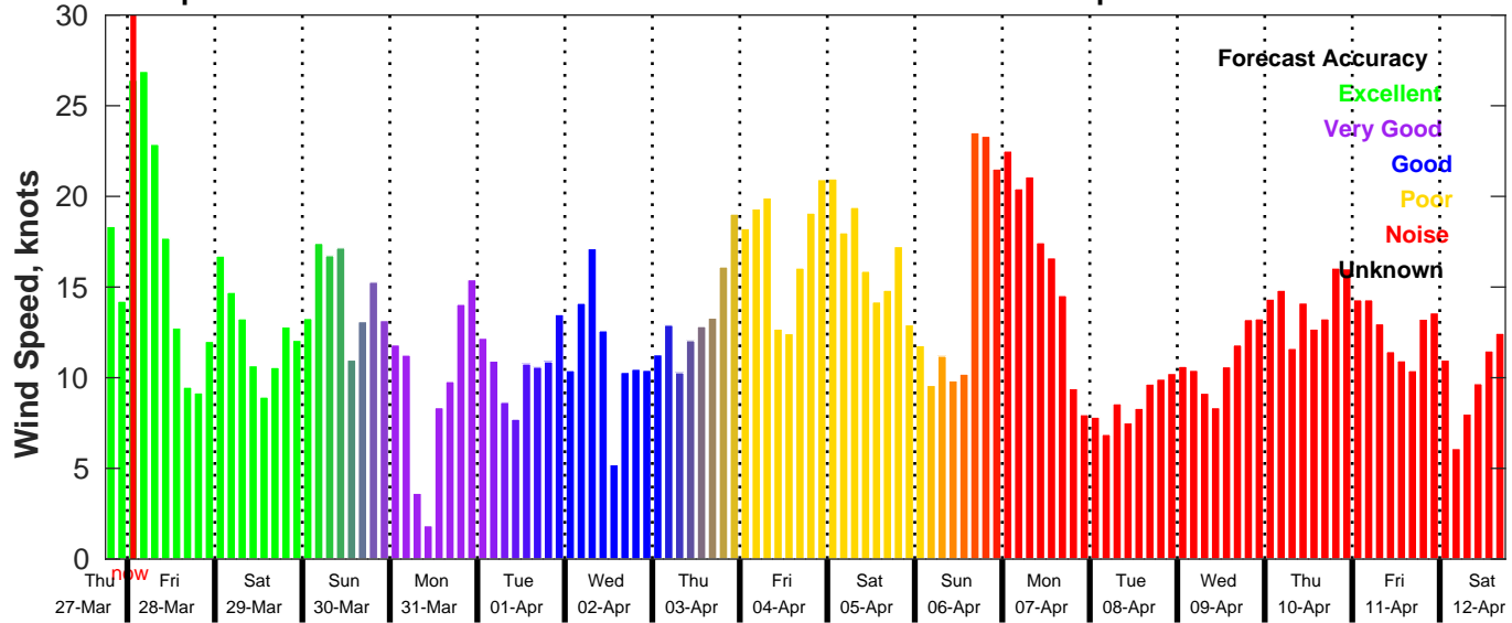
GFS Wind Speed Forecast for NDBC 42020 from 27-Mar-2025 18:00:00 to 12-Apr-2025 18:00:00
