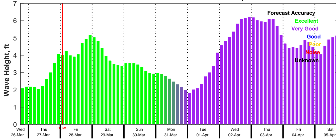
CMEMS Wave Forecast for NDBC 42035 from 26-Mar-2025 18:00:00 to 05-Apr-2025 18:00:00
