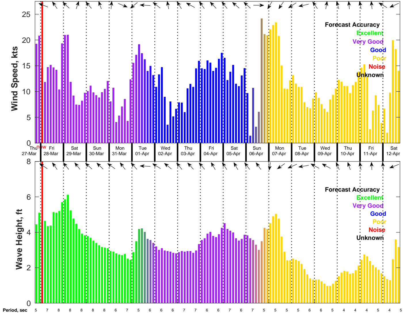
Wind & Wave Forecast for NDBC 42035 from 27-Mar-2025 18:00:00 to 12-Apr-2025 18:00:00
