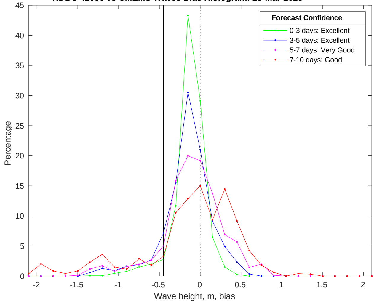
NDBC 42036 vs CMEMS Waves Bias Histogram: 28-Mar-2025
