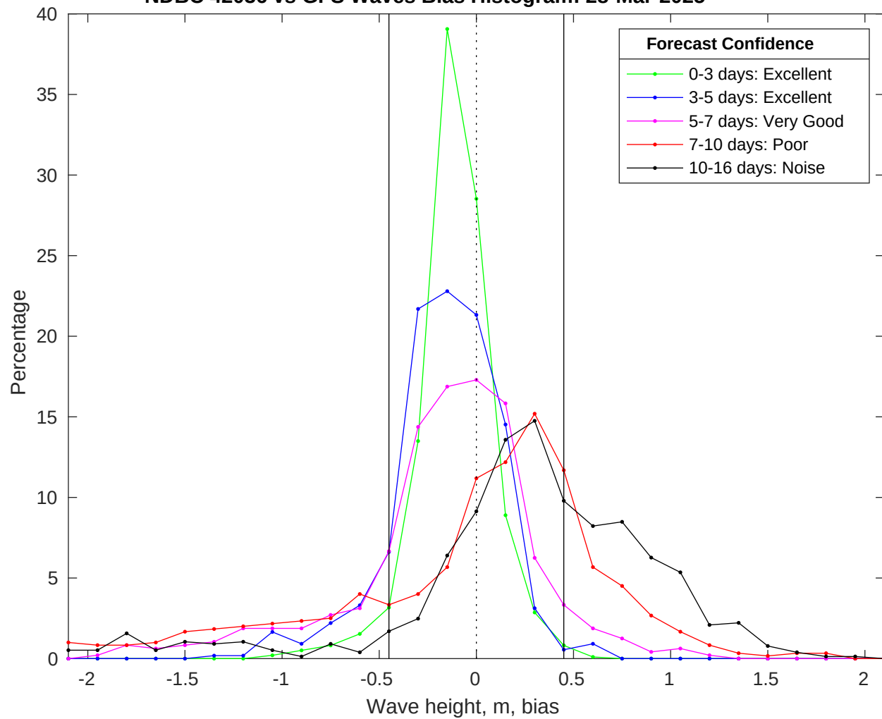
NDBC 42036 vs GFS Waves Bias Histogram: 28-Mar-2025
