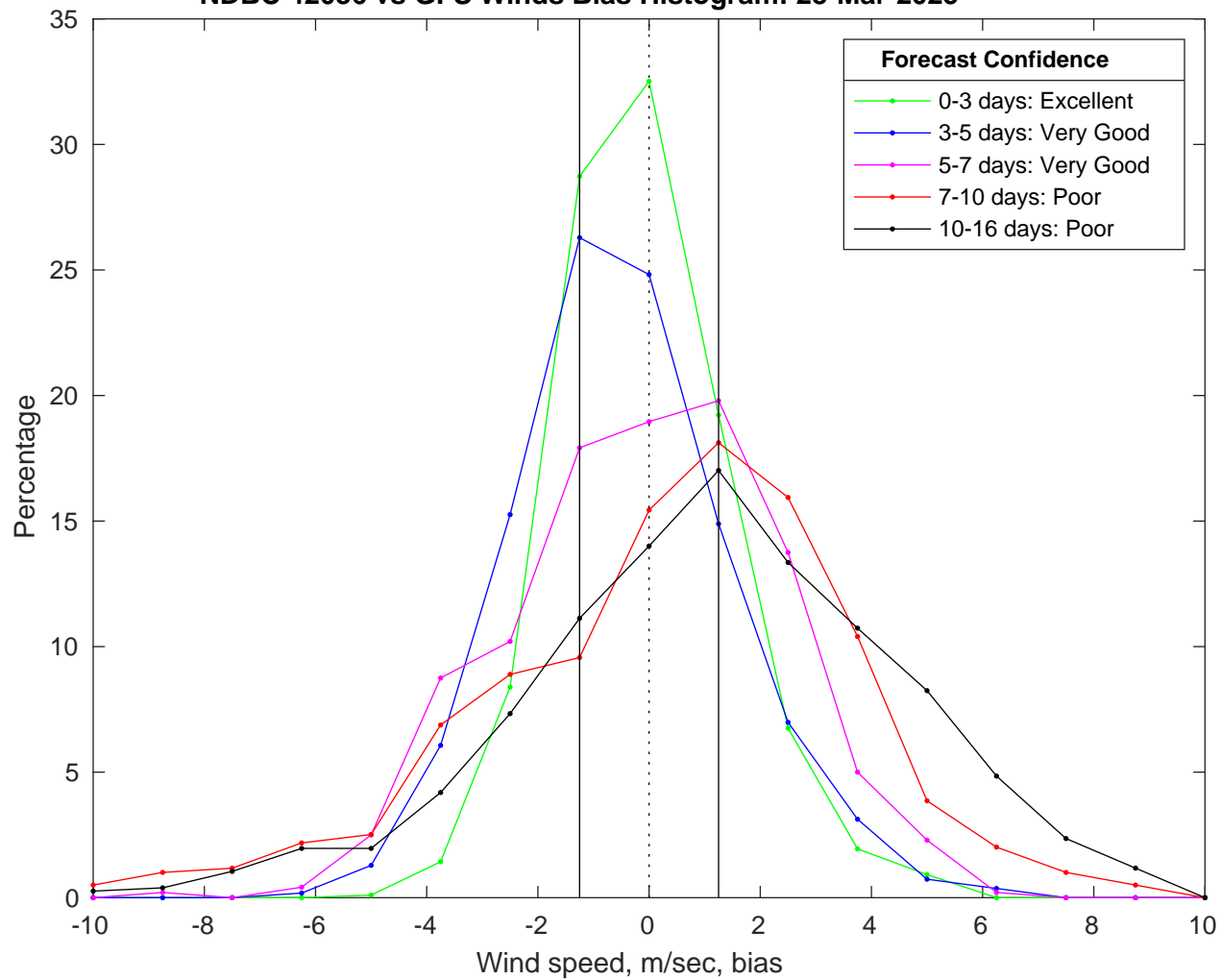
NDBC 42036 vs GFS Winds Bias Histogram: 28-Mar-2025
