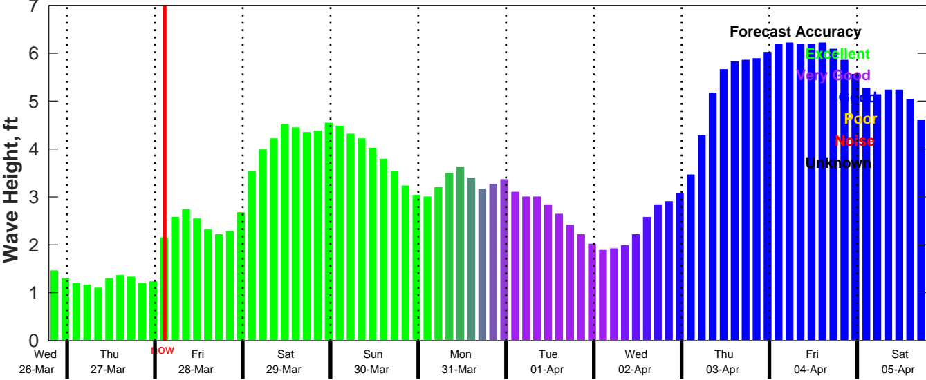
CMEMS Wave Forecast for NDBC 42036 from 26-Mar-2025 19:00:00 to 05-Apr-2025 19:00:00
