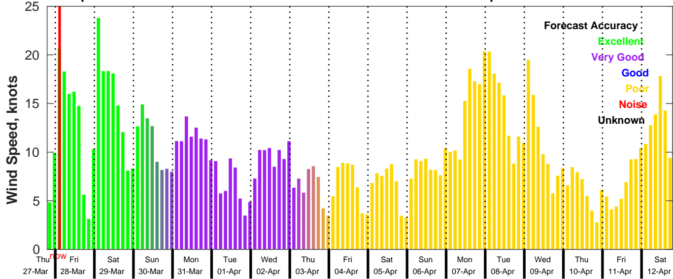
GFS Wind Speed Forecast for NDBC 42036 from 27-Mar-2025 19:00:00 to 12-Apr-2025 19:00:00
