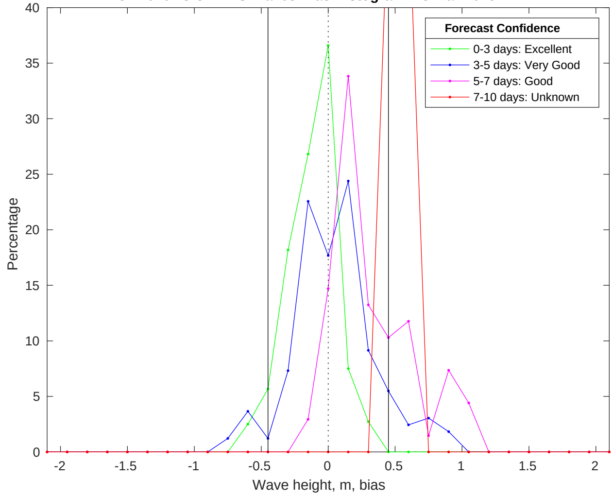
NDBC 42040 vs CMEMS Waves Bias Histogram: 28-Mar-2025
