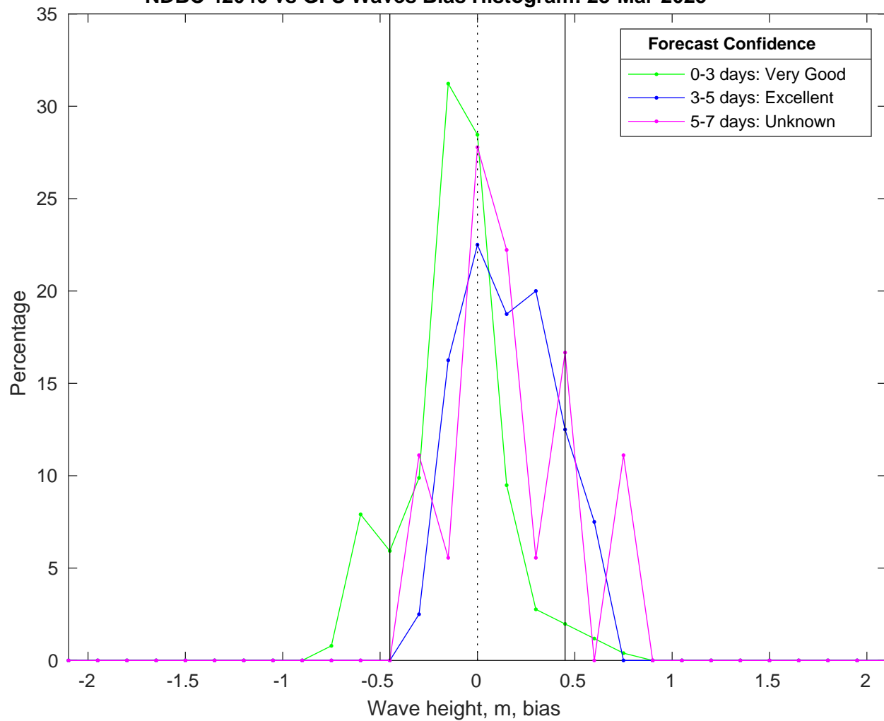
NDBC 42040 vs GFS Waves Bias Histogram: 28-Mar-2025
