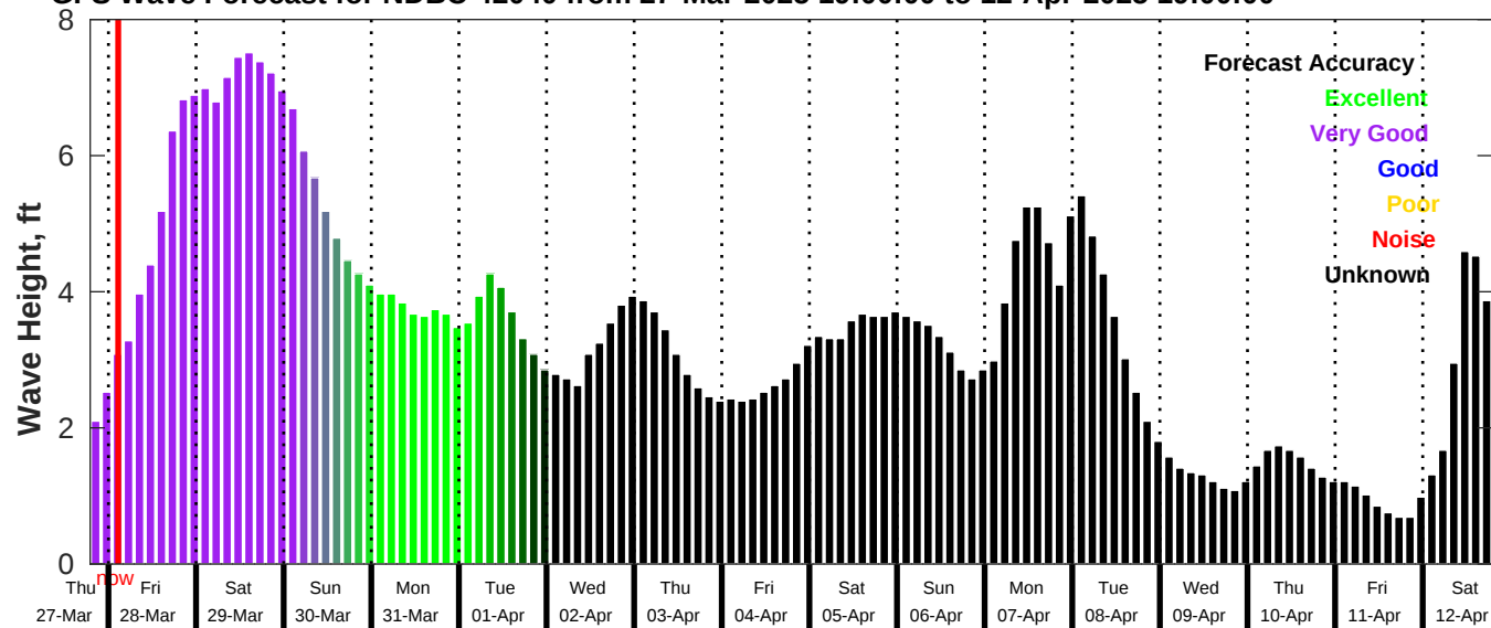
GFS Wave Forecast for NDBC 42040 from 27-Mar-2025 19:00:00 to 12-Apr-2025 19:00:00
