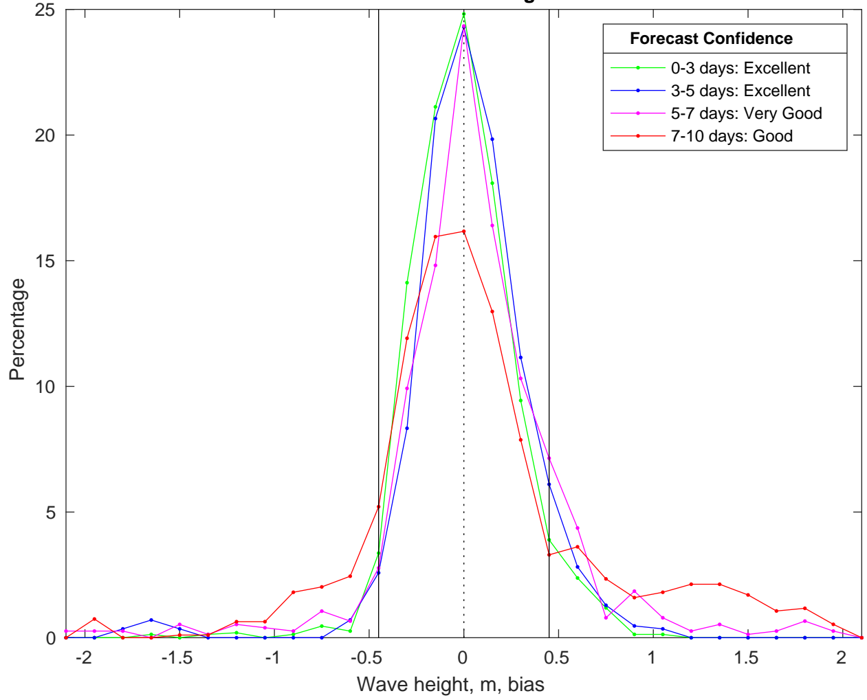
NDBC 46011 vs CMEMS Waves Bias Histogram: 28-Mar-2025
