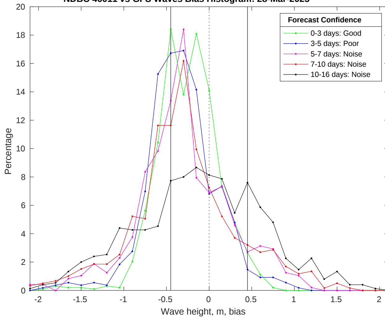
NDBC 46011 vs GFS Waves Bias Histogram: 28-Mar-2025
