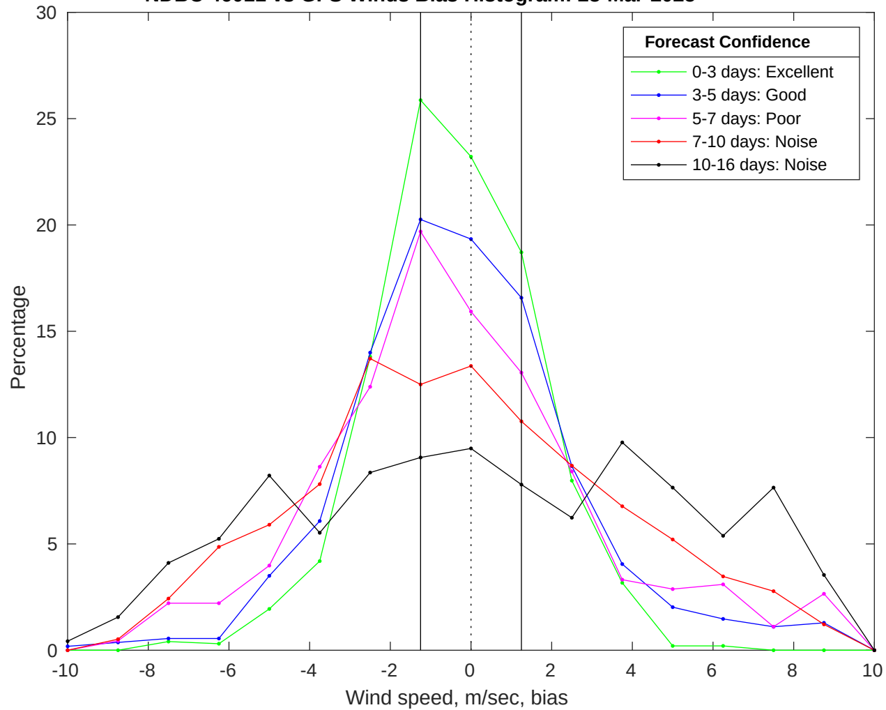
NDBC 46011 vs GFS Winds Bias Histogram: 28-Mar-2025
