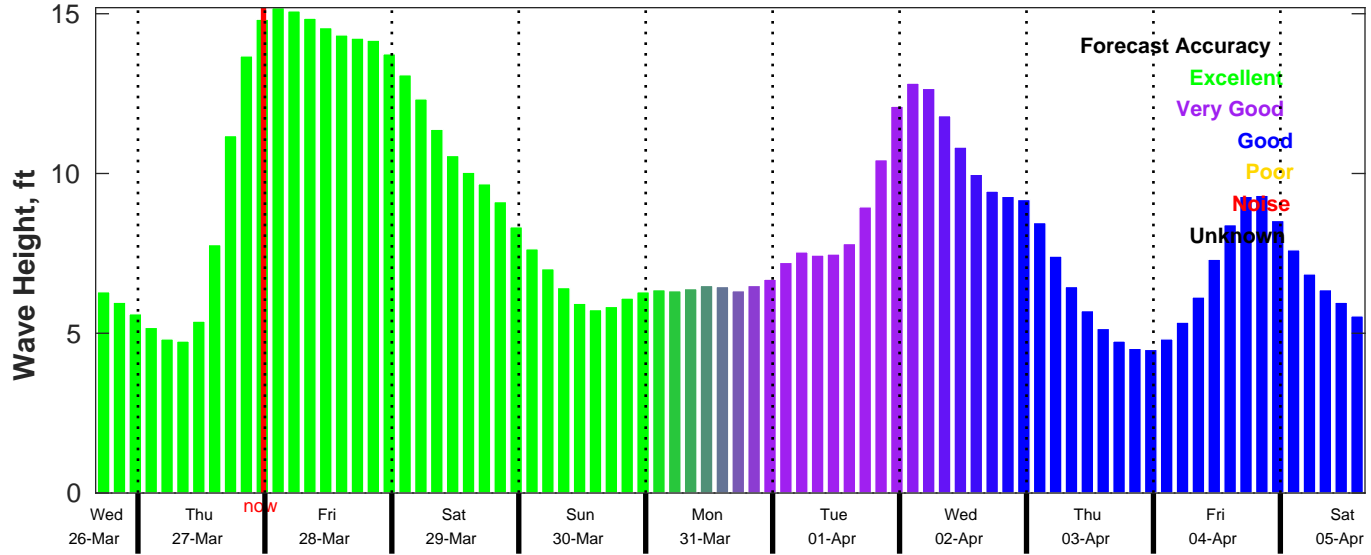
CMEMS Wave Forecast for NDBC 46011 from 26-Mar-2025 16:00:00 to 05-Apr-2025 16:00:00
