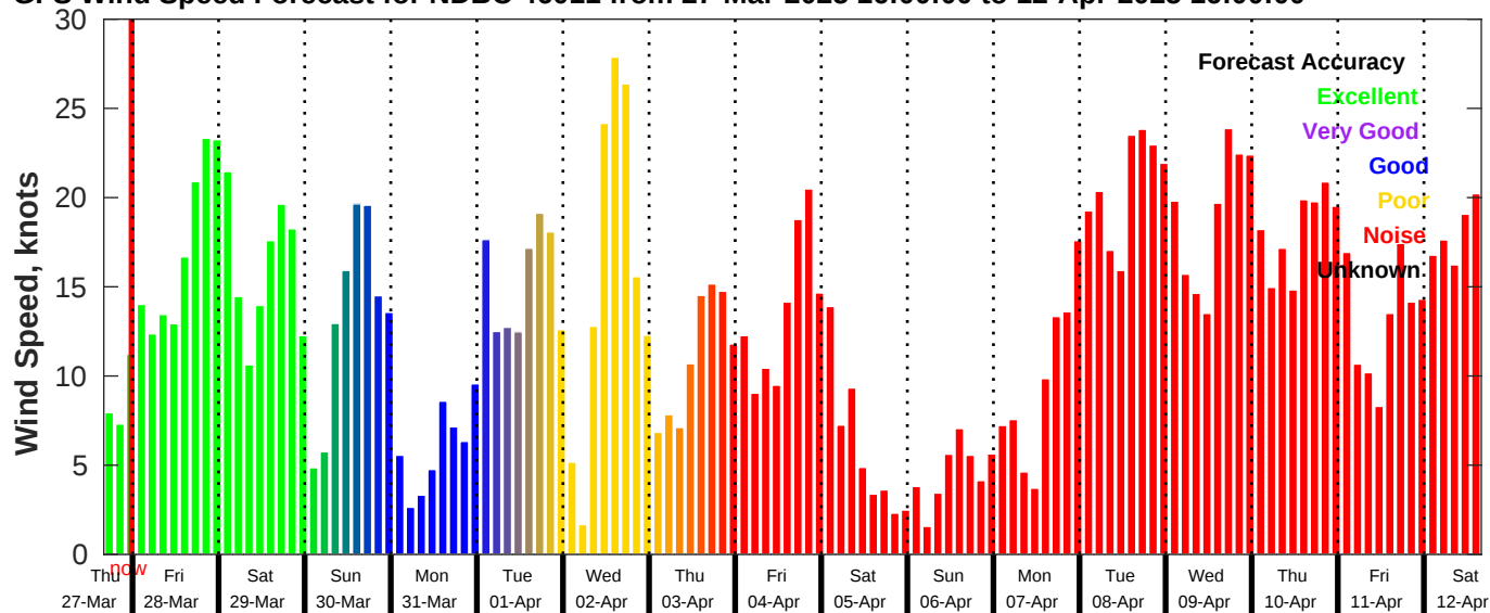
GFS Wind Speed Forecast for NDBC 46011 from 27-Mar-2025 16:00:00 to 12-Apr-2025 16:00:00
