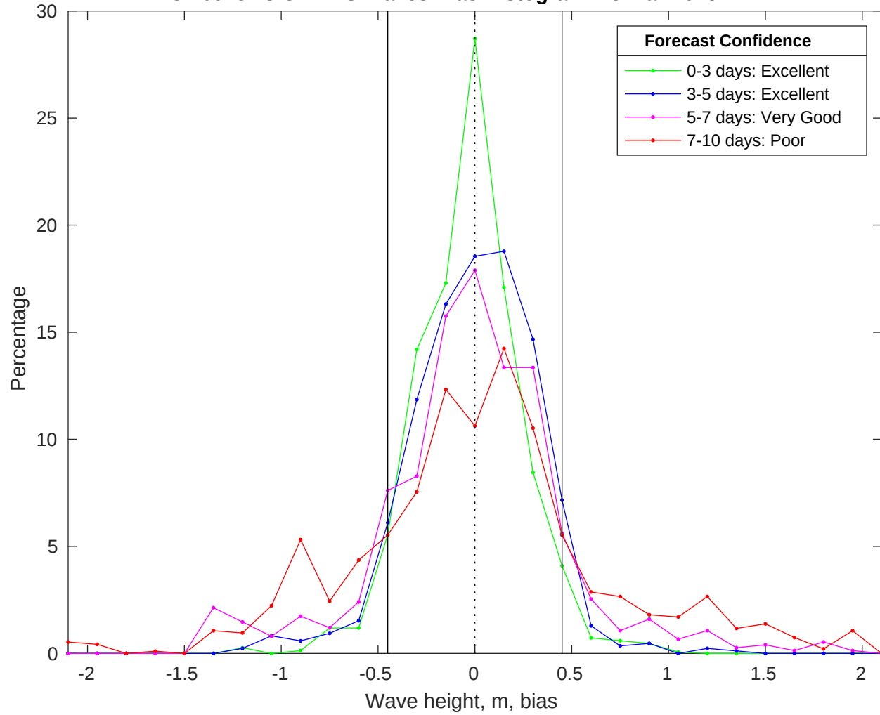
NDBC 46028 vs CMEMS Waves Bias Histogram: 28-Mar-2025
