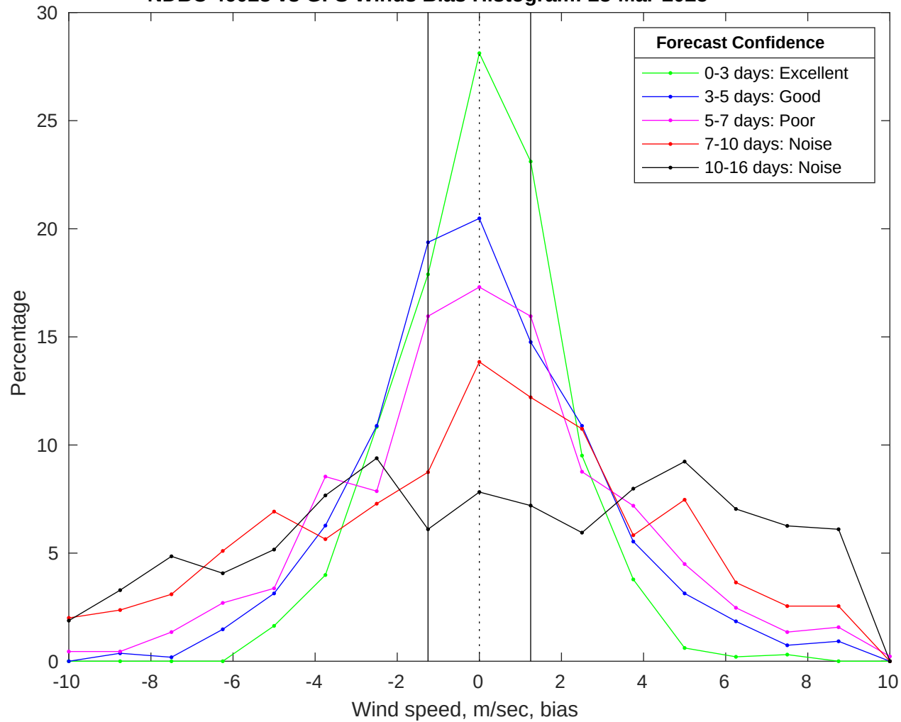
NDBC 46028 vs GFS Winds Bias Histogram: 28-Mar-2025
