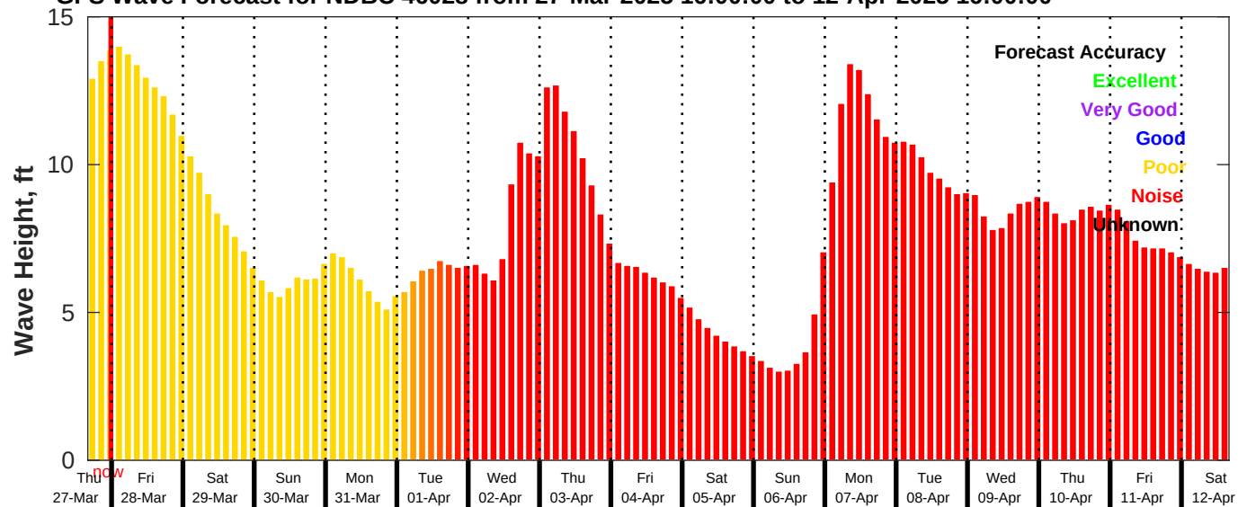
GFS Wave Forecast for NDBC 46028 from 27-Mar-2025 16:00:00 to 12-Apr-2025 16:00:00
