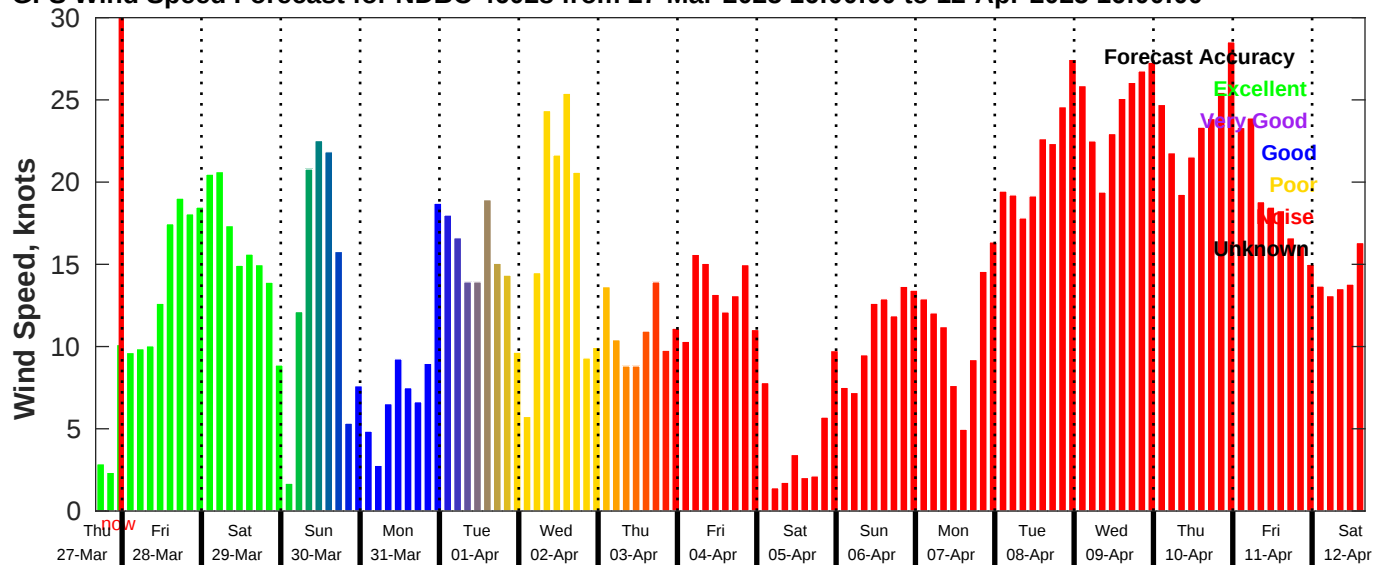
GFS Wind Speed Forecast for NDBC 46028 from 27-Mar-2025 16:00:00 to 12-Apr-2025 16:00:00
