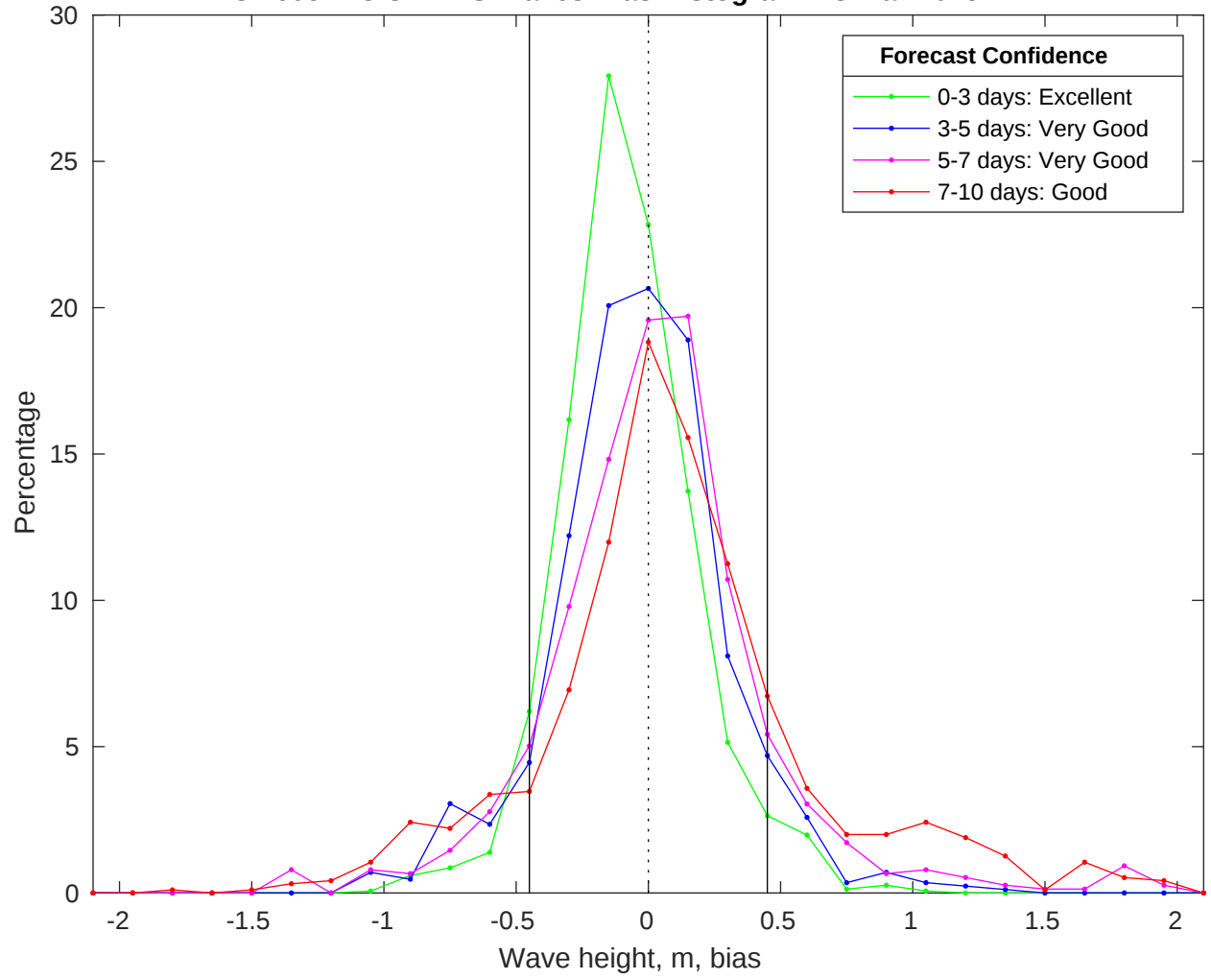
NDBC 46054 vs CMEMS Waves Bias Histogram: 28-Mar-2025
