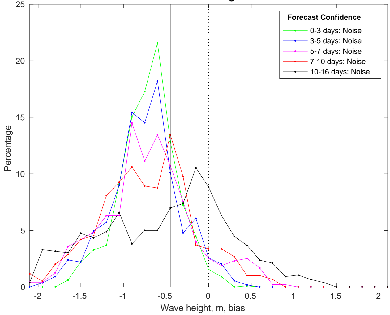
NDBC 46054 vs GFS Waves Bias Histogram: 28-Mar-2025
