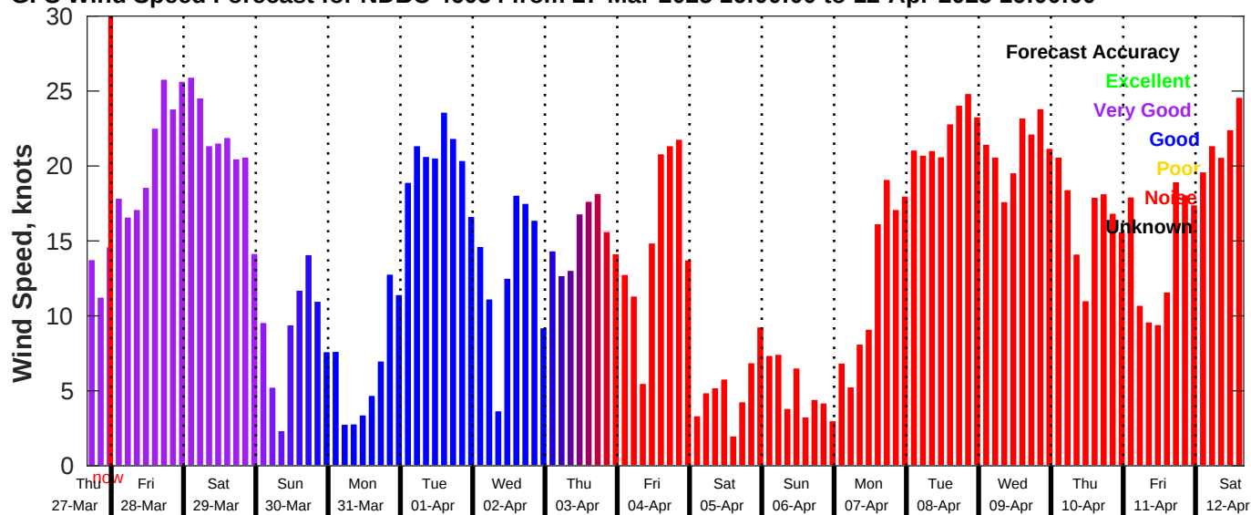
GFS Wind Speed Forecast for NDBC 46054 from 27-Mar-2025 16:00:00 to 12-Apr-2025 16:00:00
