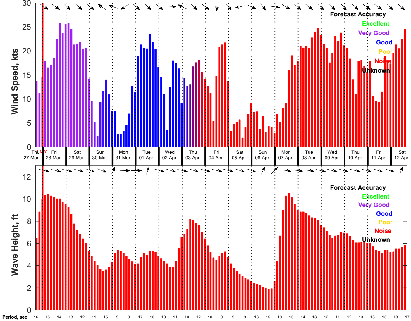
Wind & Wave Forecast for NDBC 46054 from 27-Mar-2025 16:00:00 to 12-Apr-2025 16:00:00
