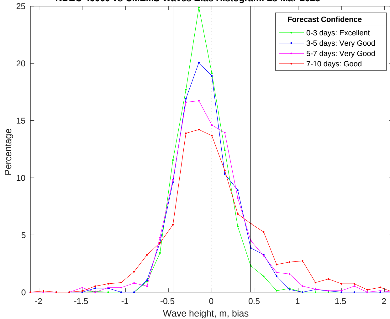
NDBC 46069 vs CMEMS Waves Bias Histogram: 28-Mar-2025
