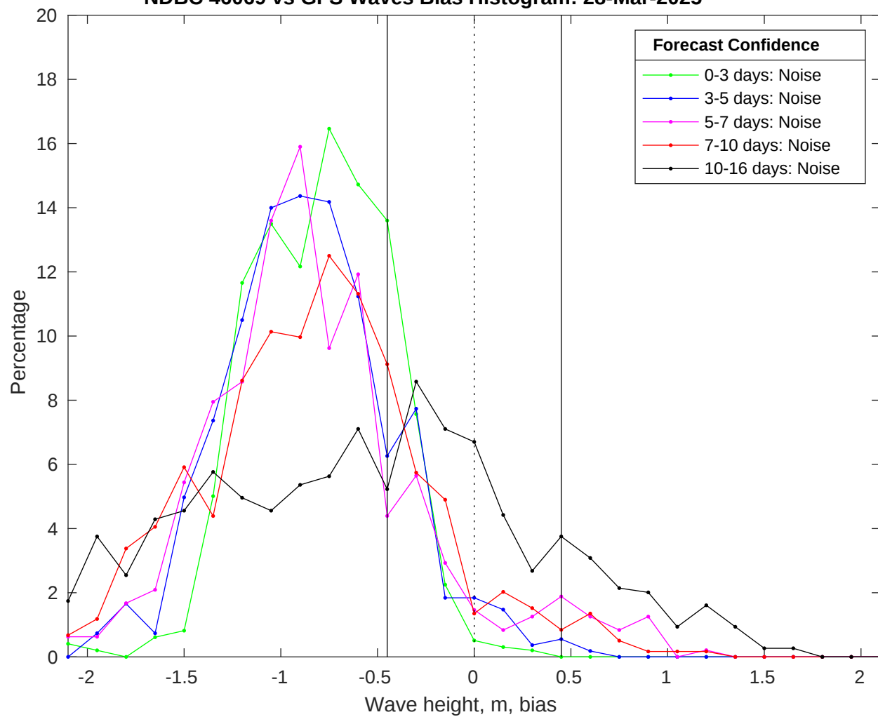
NDBC 46069 vs GFS Waves Bias Histogram: 28-Mar-2025
