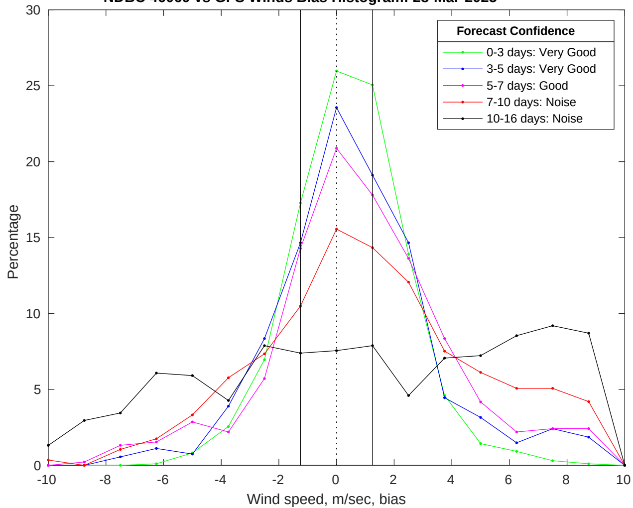
NDBC 46069 vs GFS Winds Bias Histogram: 28-Mar-2025
