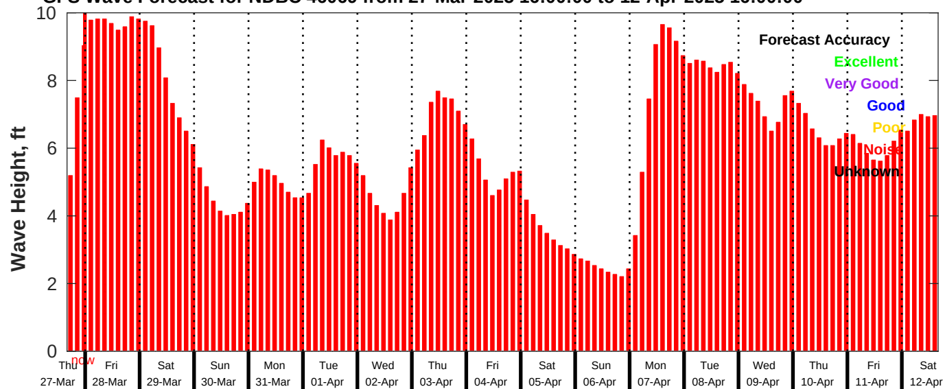
GFS Wave Forecast for NDBC 46069 from 27-Mar-2025 16:00:00 to 12-Apr-2025 16:00:00
