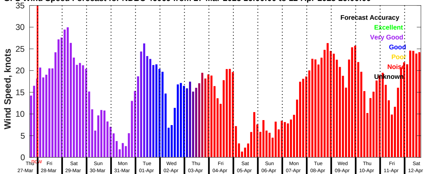
GFS Wind Speed Forecast for NDBC 46069 from 27-Mar-2025 16:00:00 to 12-Apr-2025 16:00:00
