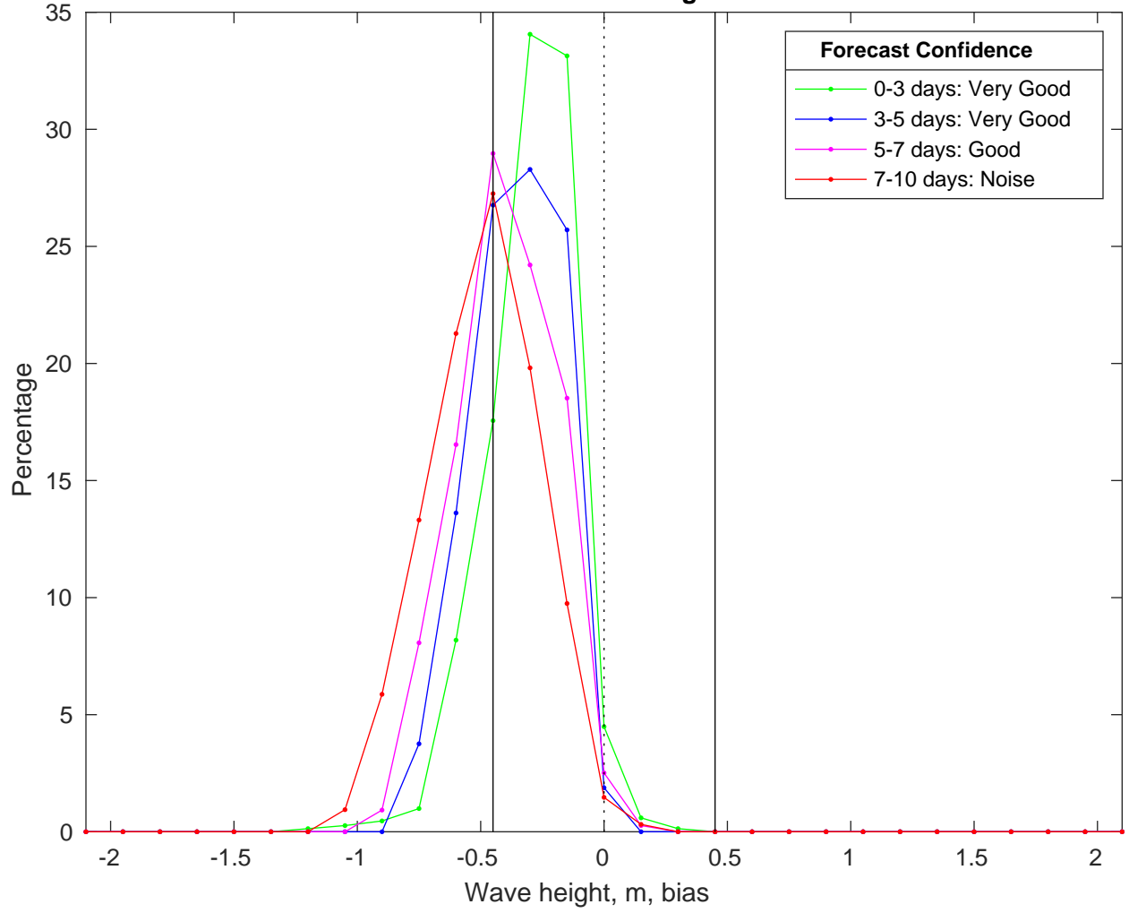
NDBC 51209 vs CMEMS Waves Bias Histogram: 28-Mar-2025
