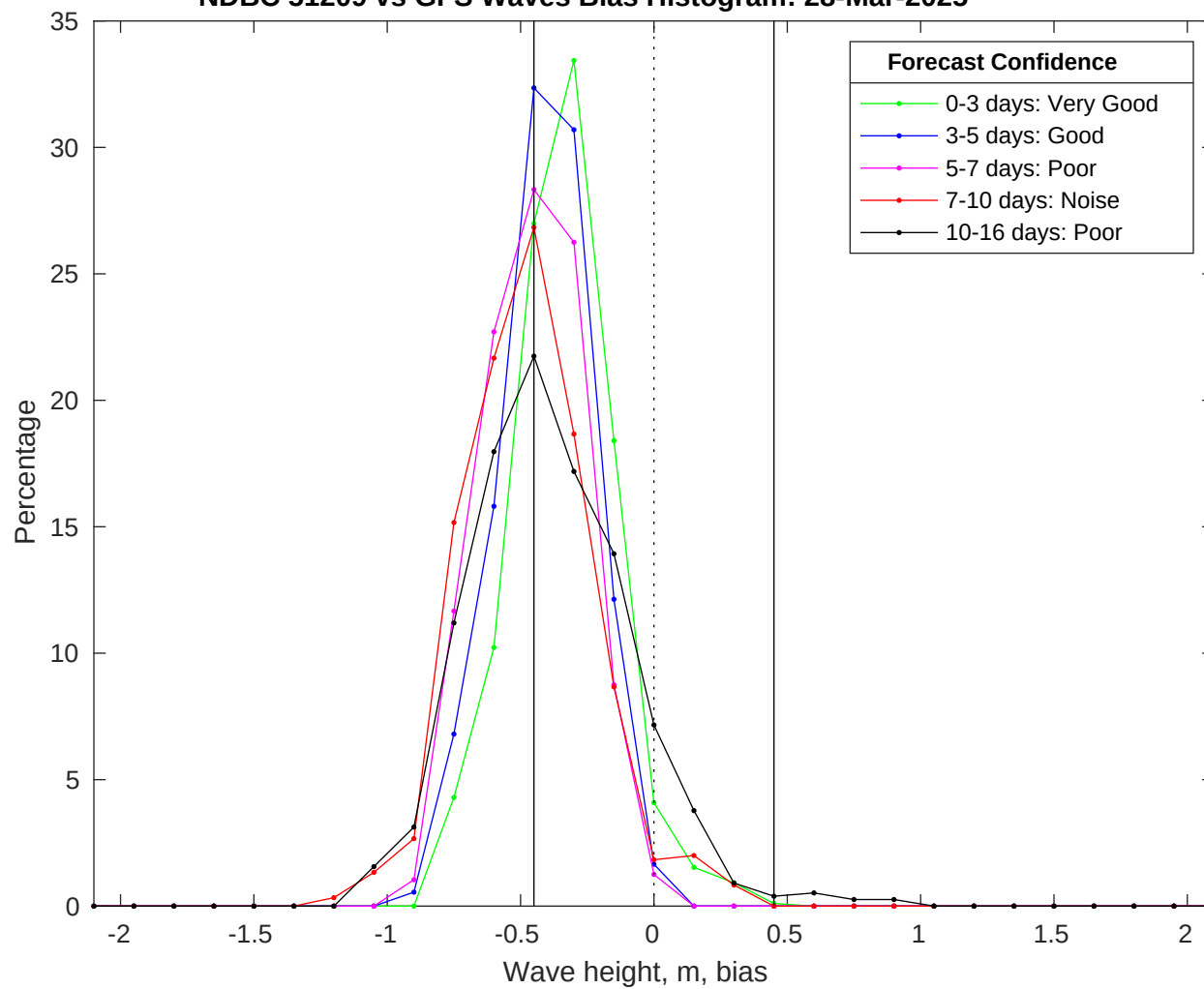
NDBC 51209 vs GFS Waves Bias Histogram: 28-Mar-2025
