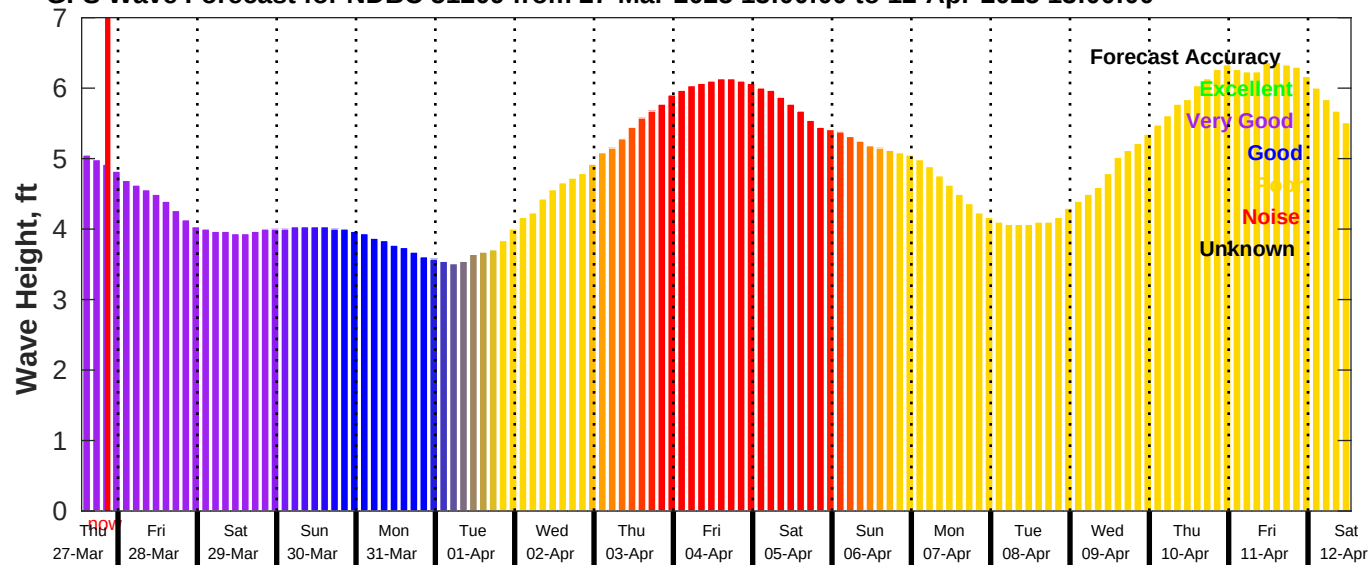
GFS Wave Forecast for NDBC 51209 from 27-Mar-2025 13:00:00 to 12-Apr-2025 13:00:00
