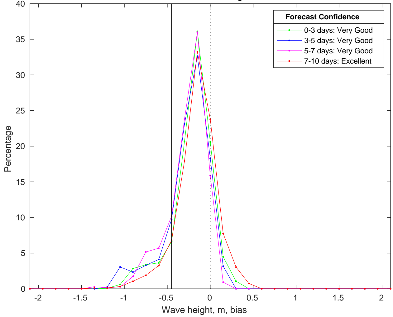
NDBC 52211 vs CMEMS Waves Bias Histogram: 28-Mar-2025
