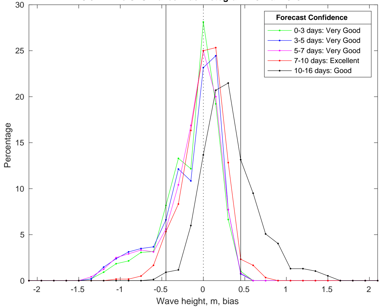
NDBC 52211 vs GFS Waves Bias Histogram: 28-Mar-2025
