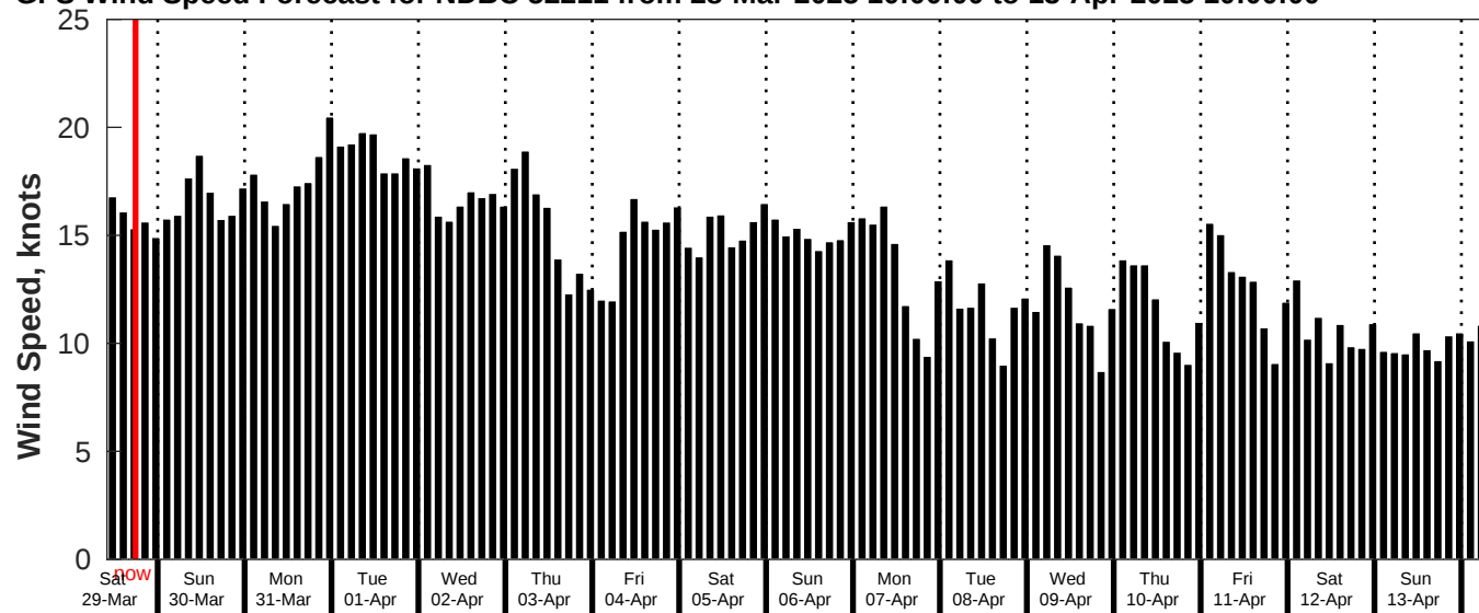
GFS Wind Speed Forecast for NDBC 52211 from 28-Mar-2025 10:00:00 to 13-Apr-2025 10:00:00
