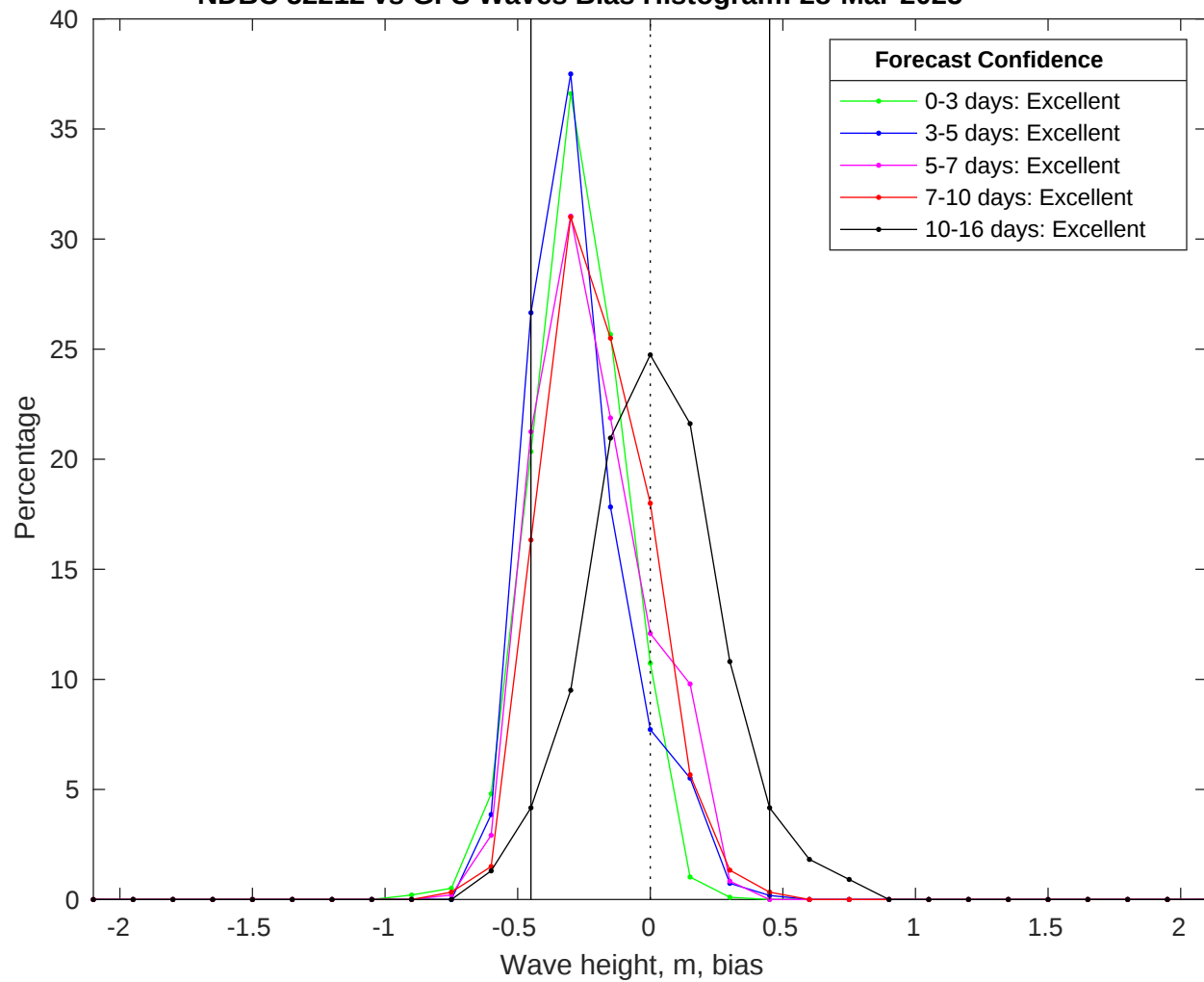
NDBC 52212 vs GFS Waves Bias Histogram: 28-Mar-2025
