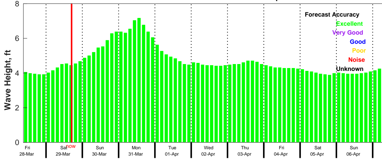
CMEMS Wave Forecast for NDBC 52212 from 27-Mar-2025 09:00:00 to 06-Apr-2025 09:00:00
