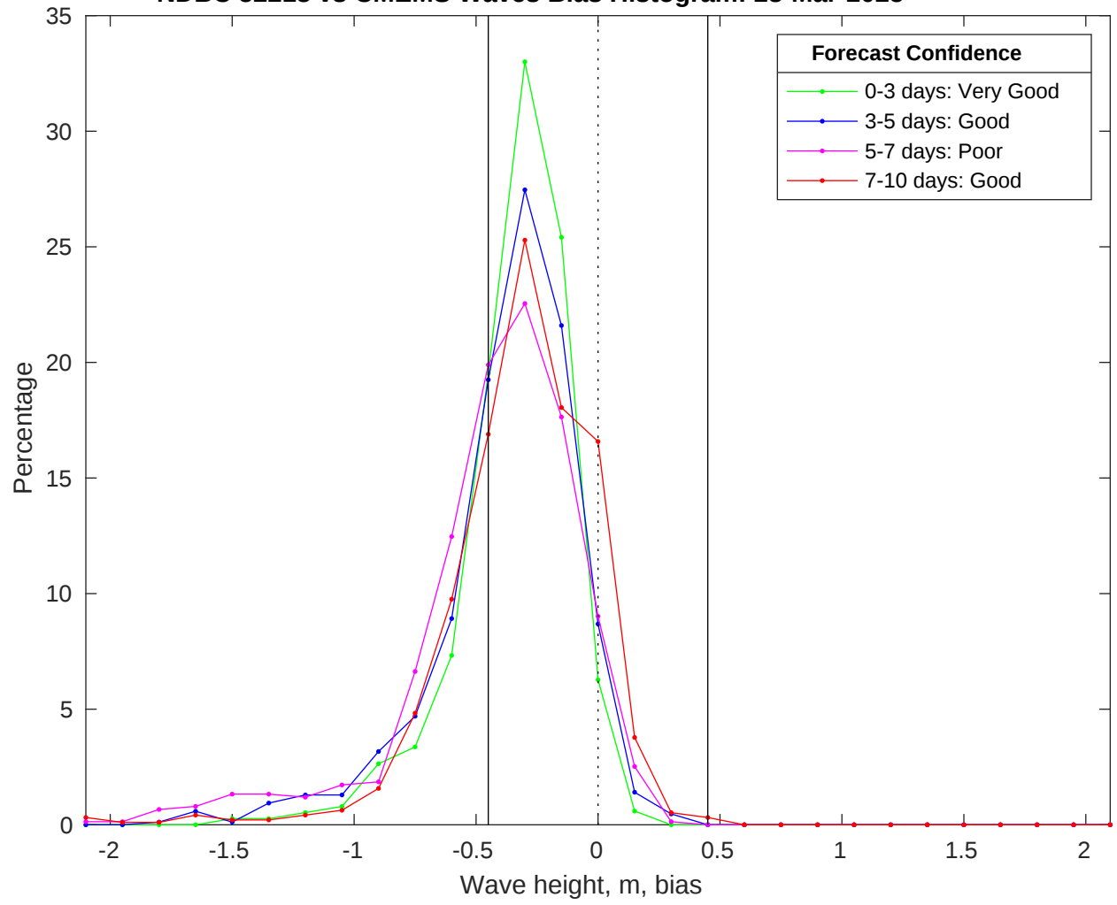
NDBC 52213 vs CMEMS Waves Bias Histogram: 28-Mar-2025
